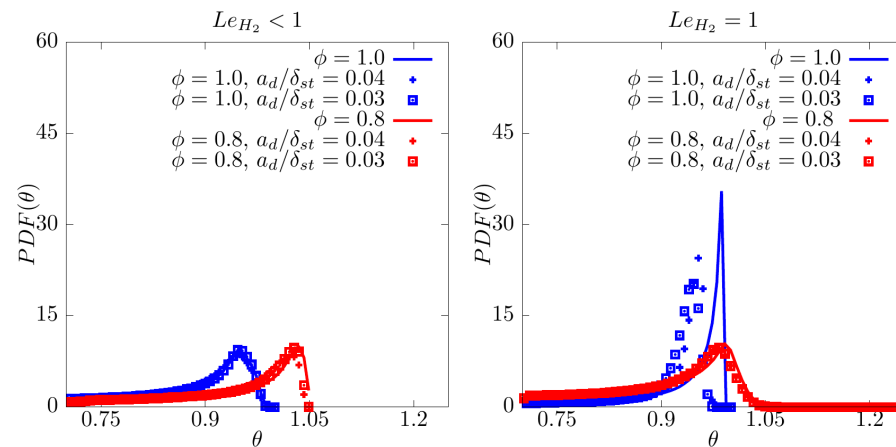
Figure 3. Probability density function of the non-dimensional temperature \theta within the reaction-dominated region of the flame c = 0.7 – 0.99 . The data are collected at t = 1.5 t_{chem} after superimposing the turbulence. The blue continuous lines and markers refer to the stoichiometric cases, while the red continuous lines and markers refer to the cases with \phi = 0.8 . The continuous lines represent the cases without water addition, and the markers refer to the cases with water addition. The different markers indicate the initial diameter of the droplets. On the left, the fuel Lewis number is Le_{H_2} < 1 , while on the right, Le_{H_2} = 1 .
