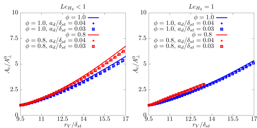
Figure 7. Flame area normalized by the flame area when the turbulence is superimposed A_c/A_{\perp}^0 versus the radius computed from the flame kernel volume r_V . The blue continuous lines and markers refer to the stoichiometric cases, while the red continuous lines and markers refer to the cases with \phi = 0.8 . The continuous lines represent the cases without water addition, and the markers refer to the cases with water addition. The different markers indicate the initial diameter of the droplets. On the left, the fuel Lewis number is Le_{H_2} < 1 , while on the right it is Le_{H_2} = 1 .
