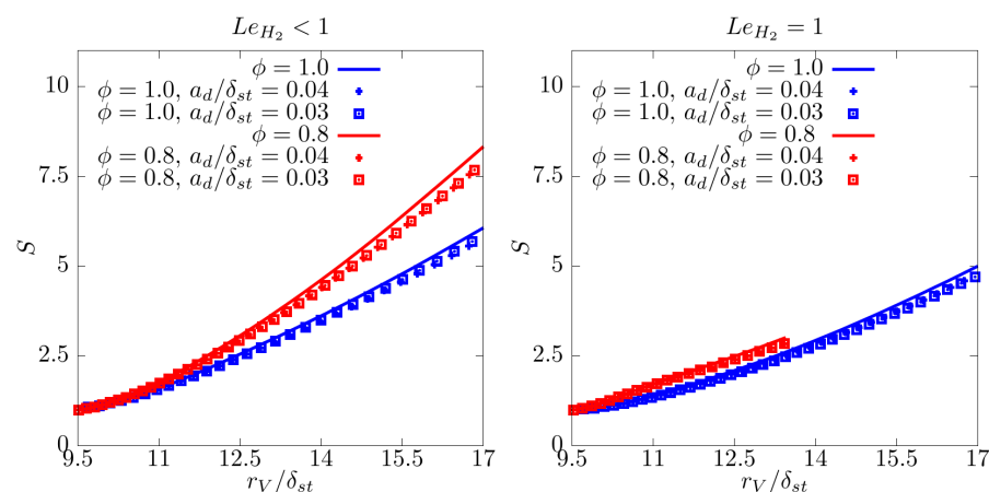
Figure 5. Evolution of the normalized total burning rate S versus the radius computed from the flame kernel volume r_V . The blue continuous lines and markers refer to the stoichiometric cases, while the red continuous lines and markers refer to the cases with \phi = 0.8 . The continuous lines represent the cases without water addition, and the markers refer to the cases with water addition. The different markers indicate the initial diameter of the droplets. On the left, the fuel Lewis number is Le_{H_2} < 1 , while on the right, Le_{H_2} = 1 .
