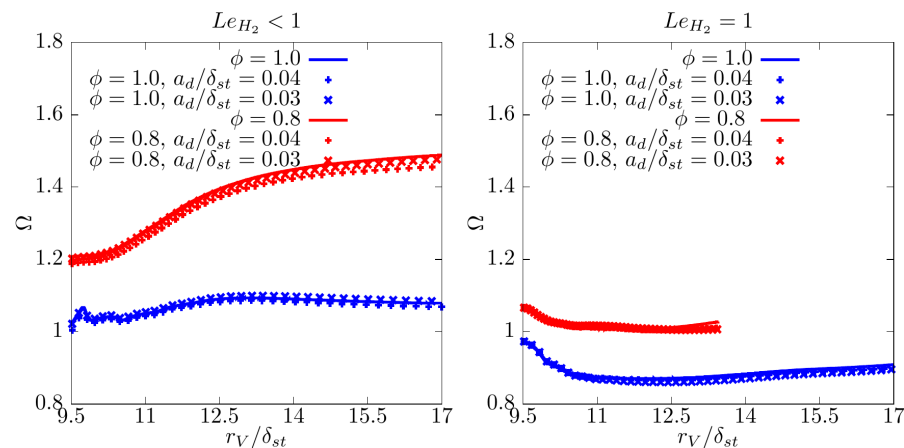
Figure 6. Burning rate per unit area normalized by the unstretched laminar equivalent \Omega versus the radius computed from the flame kernel volume r_V . The blue continuous lines and markers refer to the stoichiometric cases, while the red continuous lines and markers refer to the cases with \phi = 0.8 . The continuous lines represent the cases without water addition, and the markers refer to the cases with water addition. The different markers indicate the initial diameter of the droplets. On the left, the fuel Lewis number is Le_{H_2} < 1 , while on the right, Le_{H_2} = 1 .
