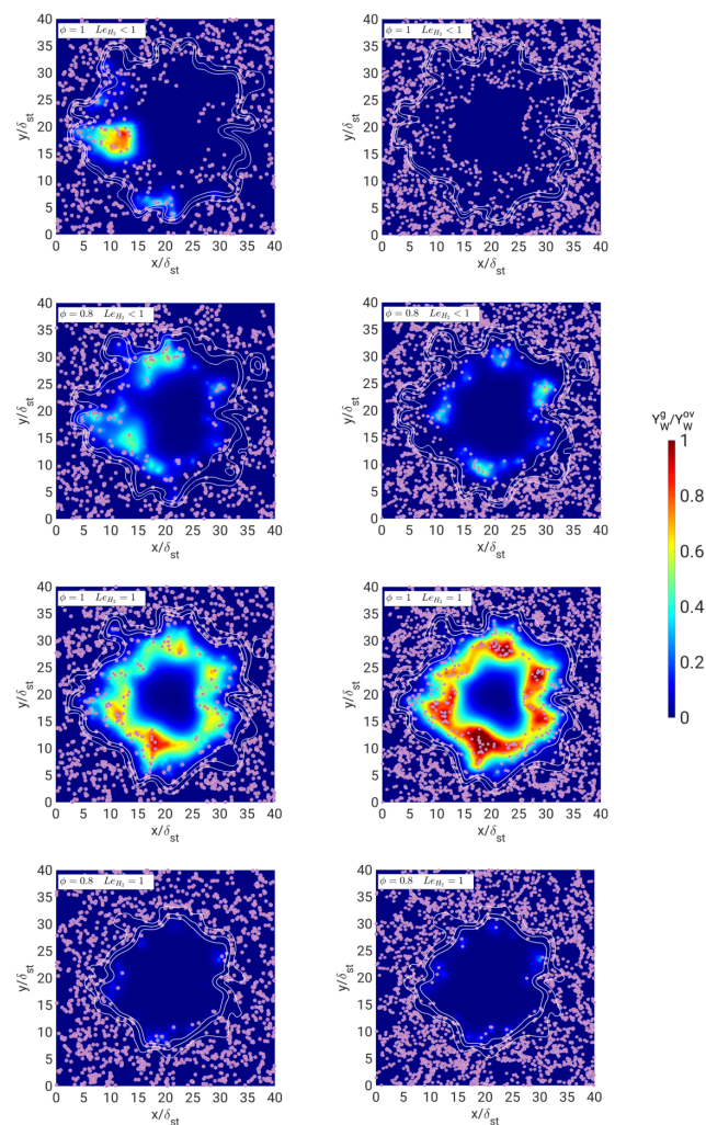
Figure 4. X – Y mid-plane of the gaseous water concentration coming only from the evaporation Y_W^g field at t = 1.5 t_{chem} after superimposing the turbulence for the cases with \phi = 1 (1st and 3rd rows) and \phi = 0.8 (2nd and 4th rows) with droplets with initial diameter a_d/\delta_{st} = 0.04 (left column) and with droplets with initial diameter a_d/\delta_{st} = 0.03 (right column). The cases with Le_{H_2} < 1 are in the first two rows, while the cases in which Le_{H_2} = 1 are in the last two rows. The white iso-lines refer to different progress variable values ( c = 0.1, 0.5 , and 0.9 ).
