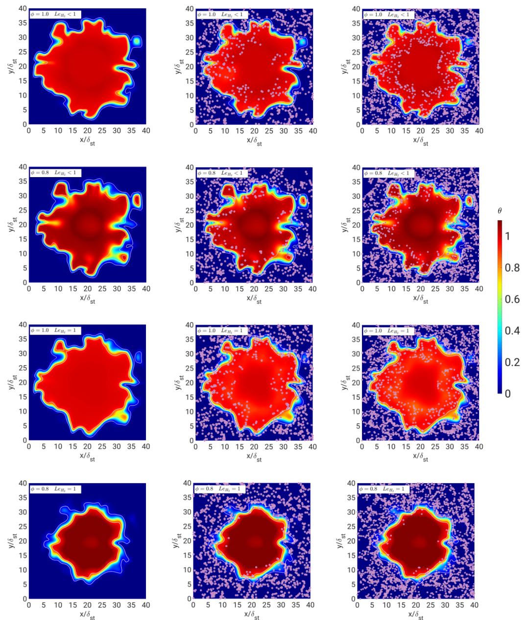
Figure 2. X - Y mid-plane of the non-dimensional temperature \theta = (\hat{T} - \hat{T}_0)/(\hat{T}_{ad,\phi} - \hat{T}_0) fields at t = 1.5 t_{chem} after superimposing the turbulence for the cases with \phi = 1 (1st and 3rd rows) and \phi = 0.8 (2nd and 4th rows) without droplets (left column), with droplets of initial diameter a_d/\delta_{st} = 0.04 (central column), and with droplets of initial diameter a_d/\delta_{st} = 0.03 (right column). The cases with Le_{H_2} < 1 are in the first two rows, while the cases in which Le_{H_2} = 1 are in the last two rows. The white iso-lines refer to different progress variable values ( c = 0.1, 0.5 , and 0.9 ).
