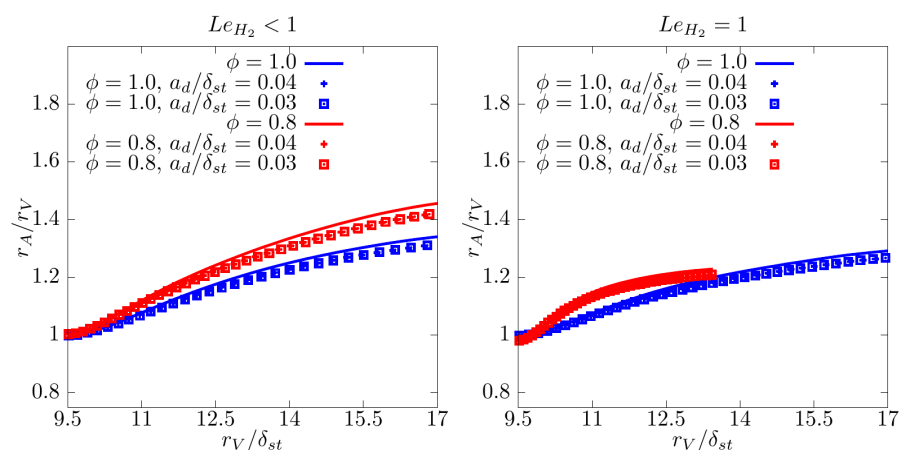
Figure 8. Flame-area-based radius normalized by volume-based radius r_A/r_V versus the radius computed from the flame kernel volume r_V . The blue continuous lines and markers refer to the stoichiometric cases, while the red continuous lines and markers refer to the cases with \phi = 0.8 . The continuous lines represent the cases without water addition, and the markers refer to the cases with water addition. The different markers indicate the initial diameter of the droplets. On the left, the fuel Lewis number is Le_{H_2} < 1 , while on the right, Le_{H_2} = 1 .
