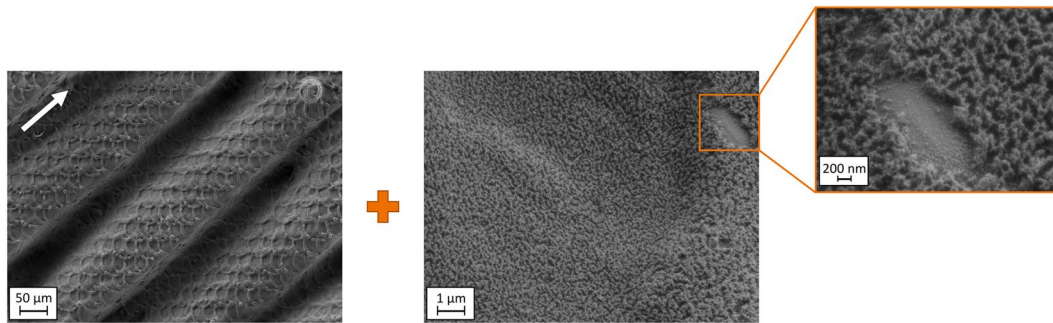
Fig. 8 SEM images of a A0-oriented Ti6Al4V surface after laser treatment
