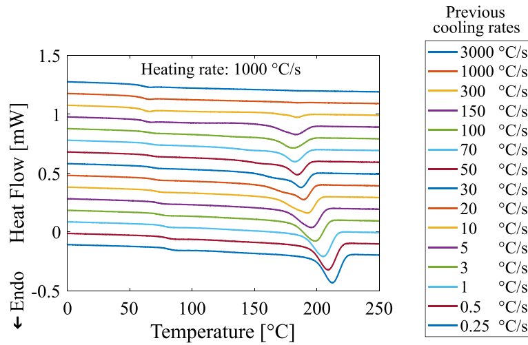
Fig. 4 Results of F-DSC heating runs after cooling with temperature rates specified
